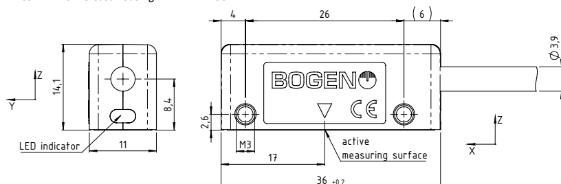
IKS9.1 - Zinc Die Cast Housing: 11 x 14.1 x 36
