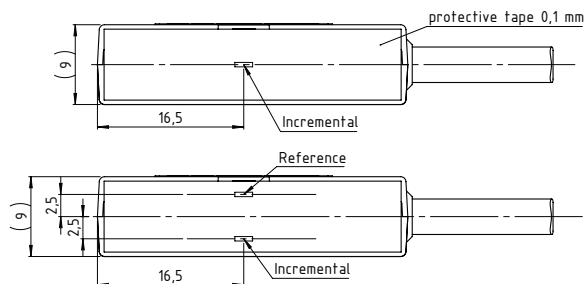
View on active measuring surface
