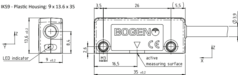
IKS9 - Plastic Housing: 9 x 13.6 x 35
